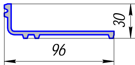
HP-376; 1,101кг/п.м.
