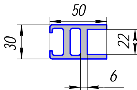
HP-436-01; 1,743кг/п.м.
