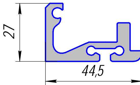
HP-517; 1,061кг/п.м.
