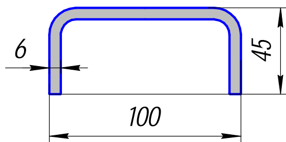
440362; 2,740кг/п.м.
