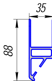
ПА-253; 1,544кг/п.м.
